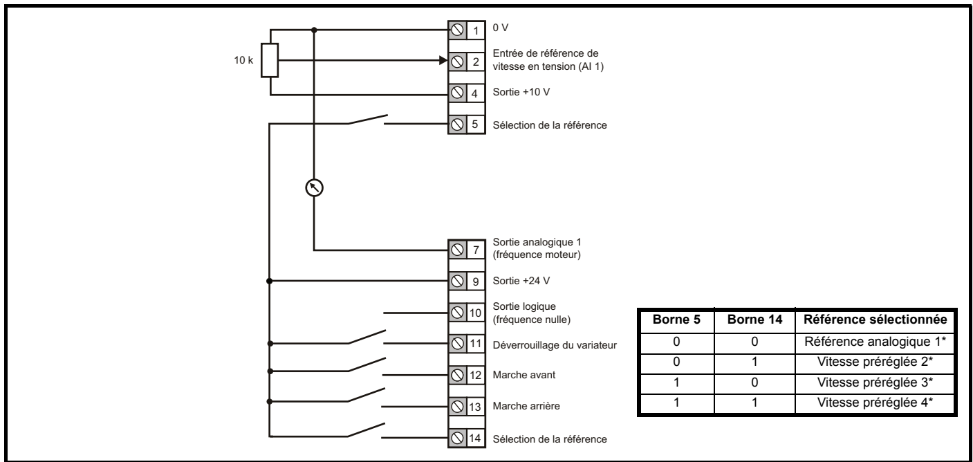
Figure 6-5 Pr 05 = AI.Pr
