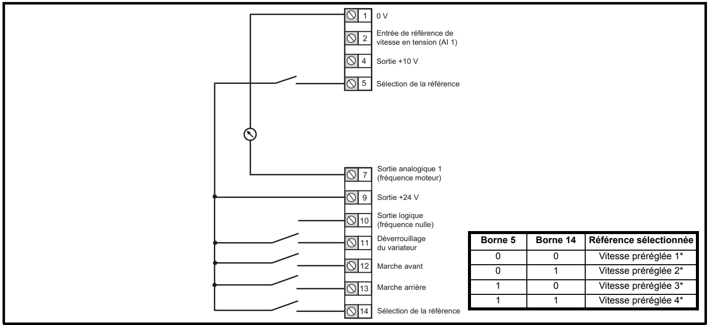
Figure 6-6 Pr 05 = PrESEt
