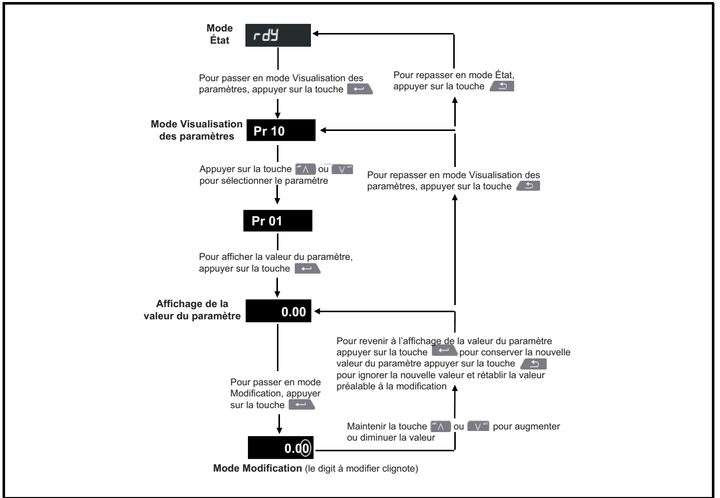
Figure 5-3 Modes Affichage
