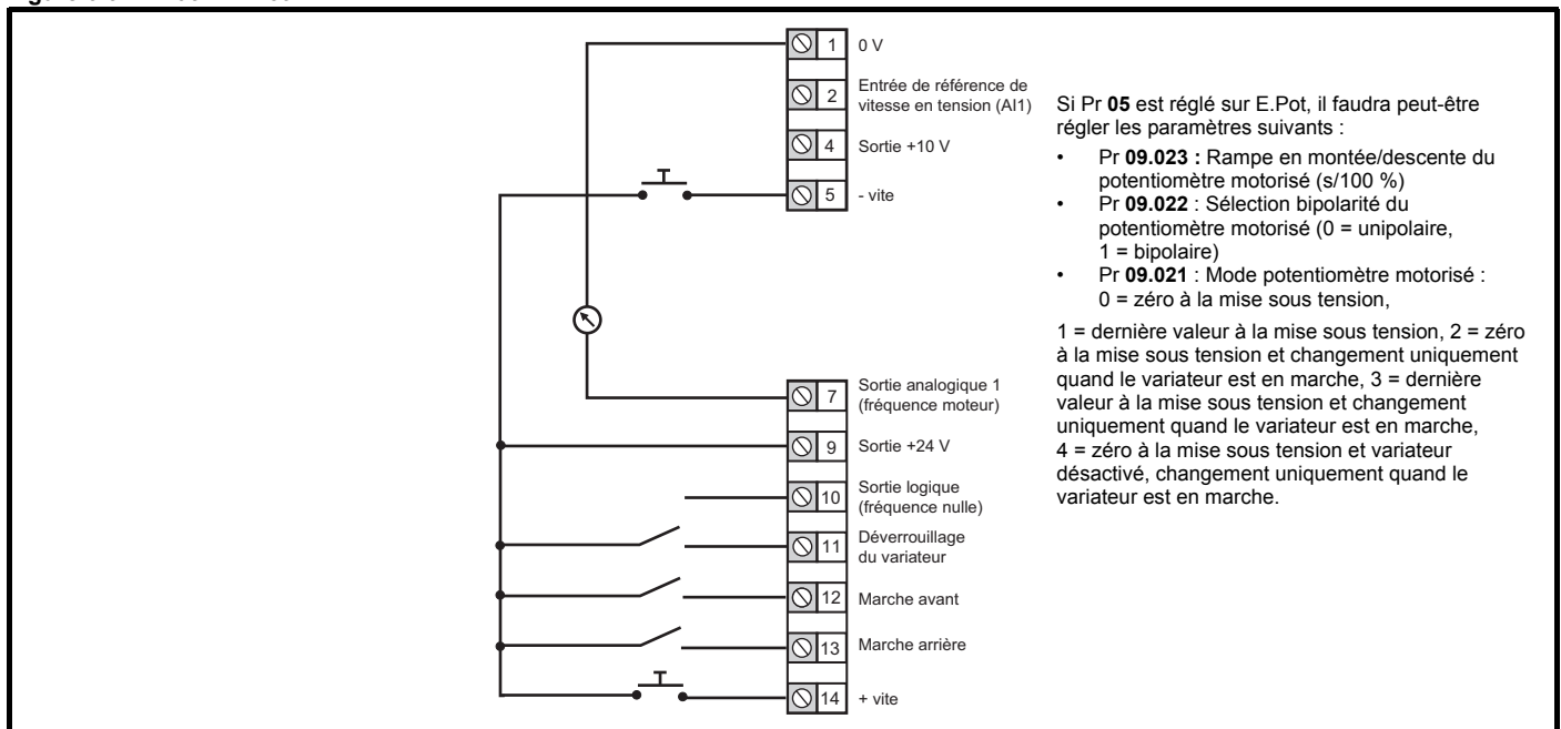
Figure 6-9 Pr 05 = E.Pot
