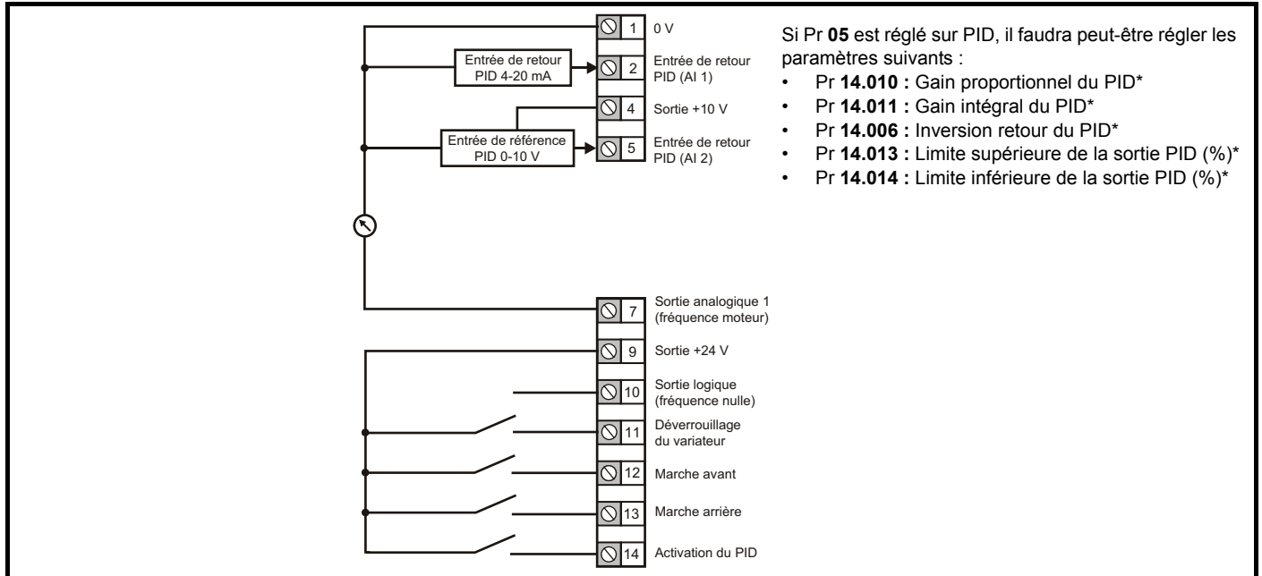
Figure 6-11 Pr 05 = Pid
