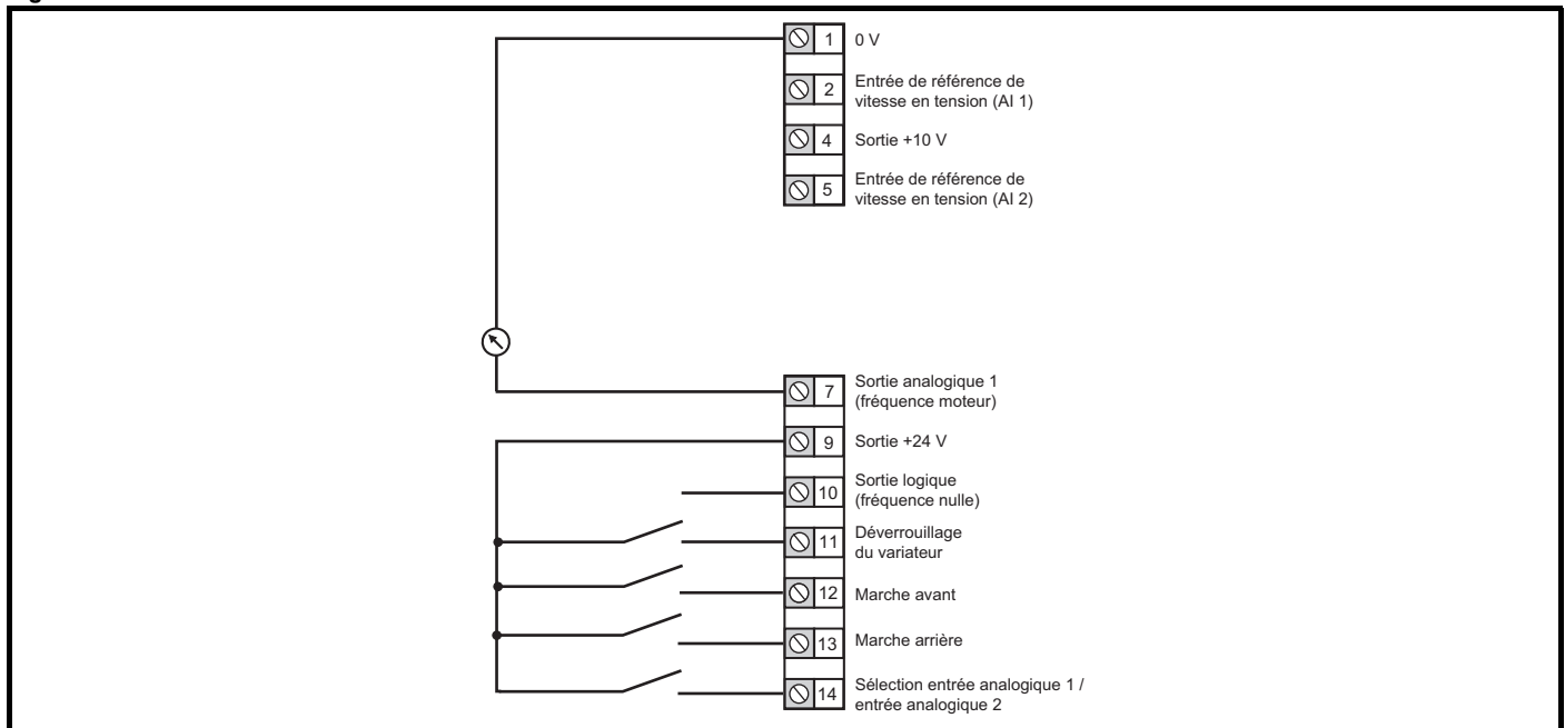
Figure 6-8 Pr 05 = PAd.rEF
